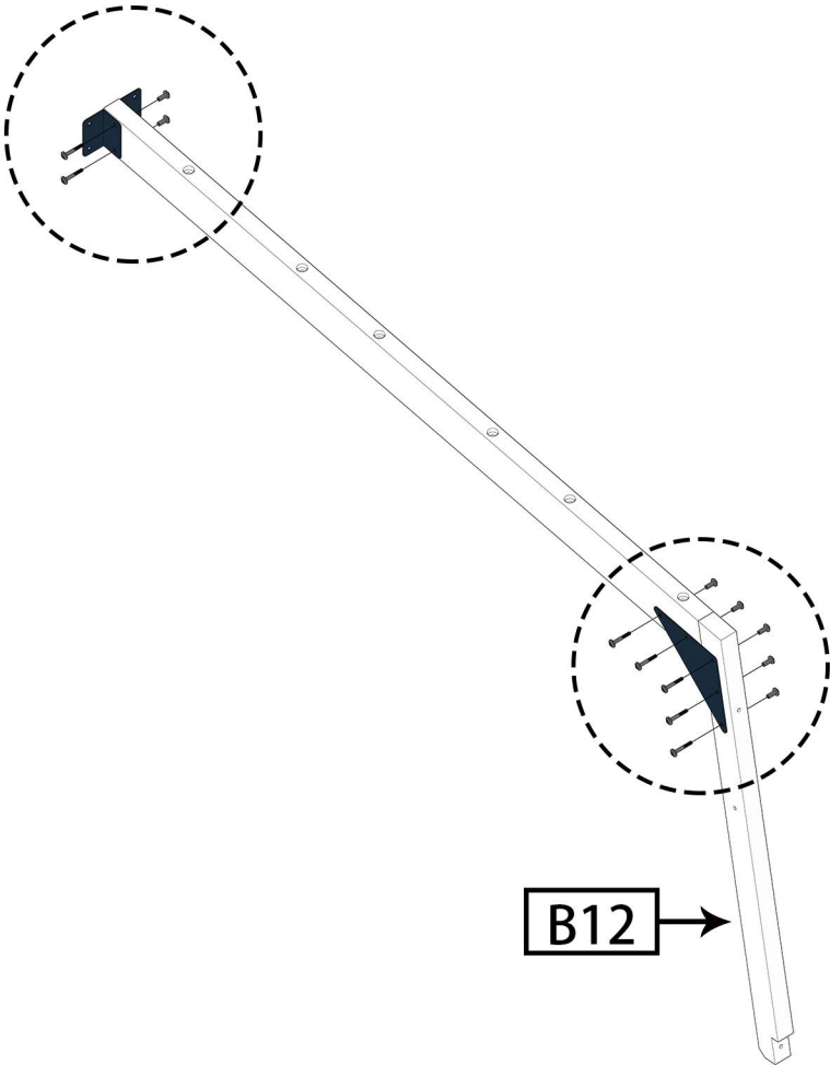
BRACKET-651003-5011
