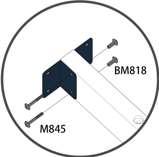
BRACKET-651003-5011
