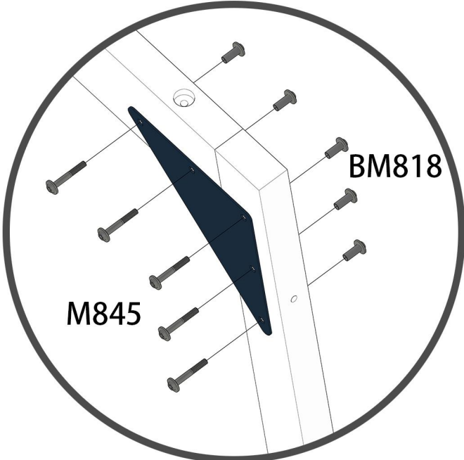
METAL BOARD-651007-5011
