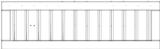
WP3 PANEL DE LA PARED - W2A03575 (x1) 1 1/16"x12 3/4"x41 5/8" (27x324x1058)
