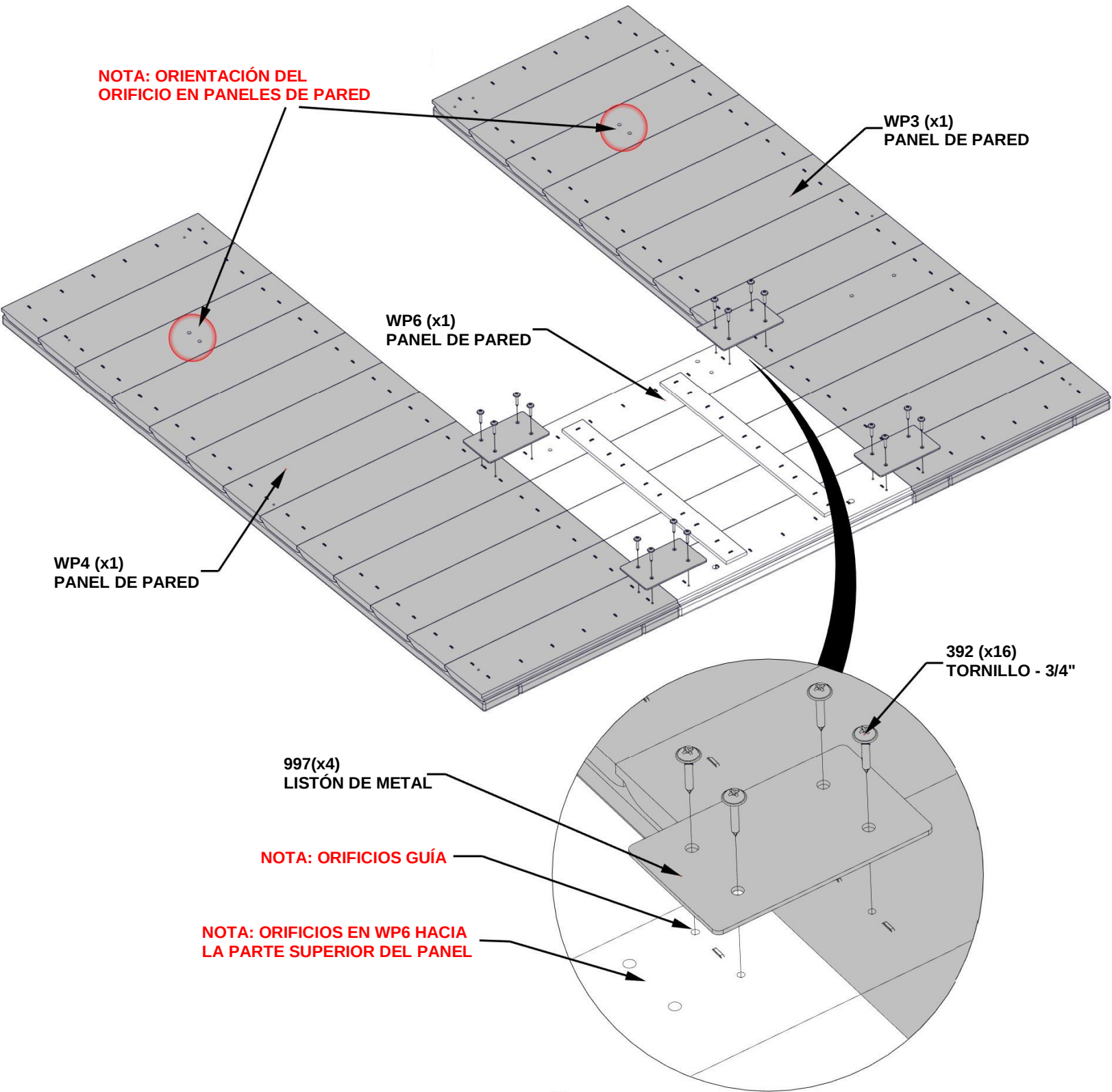
WP4 PANEL DE LA PARED - W2A03576 (x1) 1 1/16"x12 3/4"x41 5/8" (27x324x1058)
