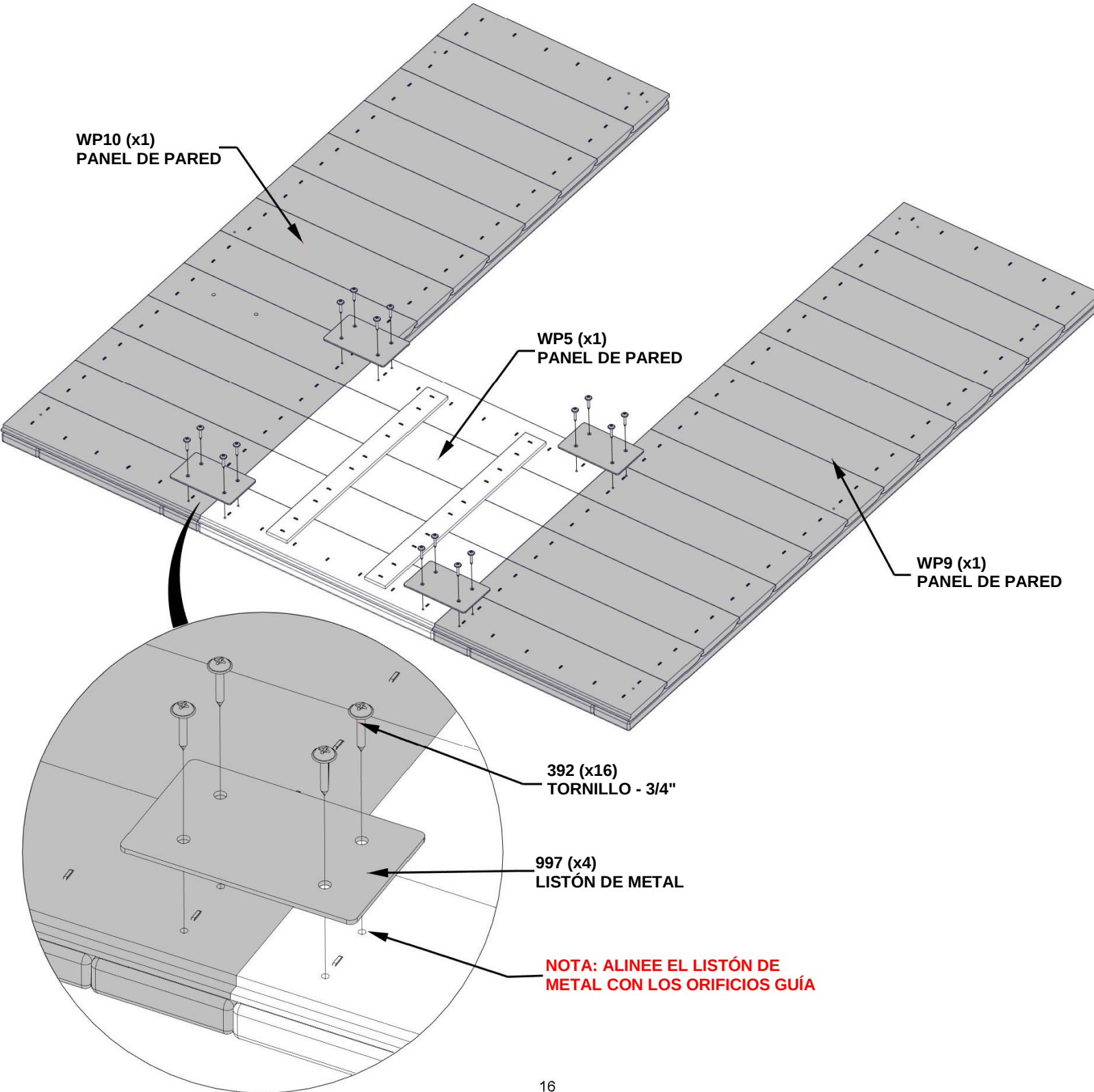
WP10 PANEL DE LA PARED - W2A03586 (x1) 1 1/16"x12 3/4"x41 5/8" (27x324x1058)
