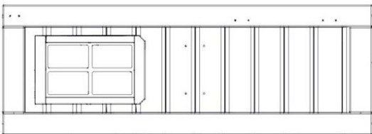
WP2 PANEL DE LA PARED - W2A03574 (x1) 3 3/8"x14"x39 3/4" (27x355x1010)
