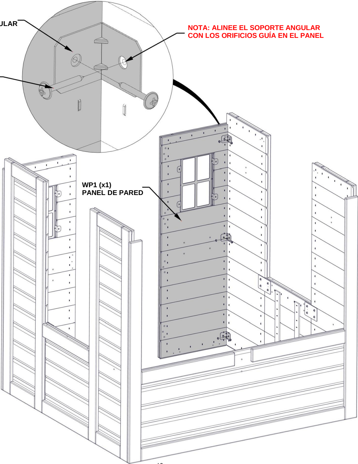
WP1 PANEL DE LA PARED - W2A03573 (x1) 3 3/8"x14"x39 3/4" (27x355x1010)
