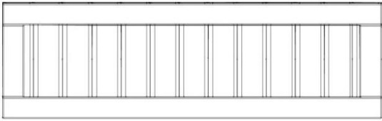
WP10 PANEL DE LA PARED - W2A03586 (x1) 1 1/16"x12 3/4"x41 5/8" (27x324x1058)
