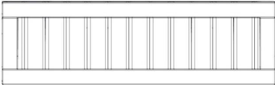
WP9 PANEL DE LA PARED - W2A03585 (x1) 1 1/16"x12 3/4"x41 5/8" (27x324x1058)
