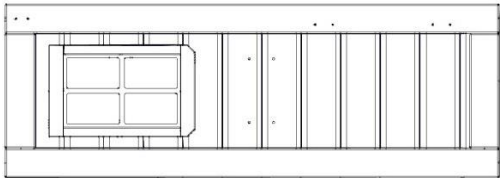
WP2 PANEL DE LA PARED - W2A03574 (x1) 3 3/8"x14"x39 3/4" (27x355x1010)
