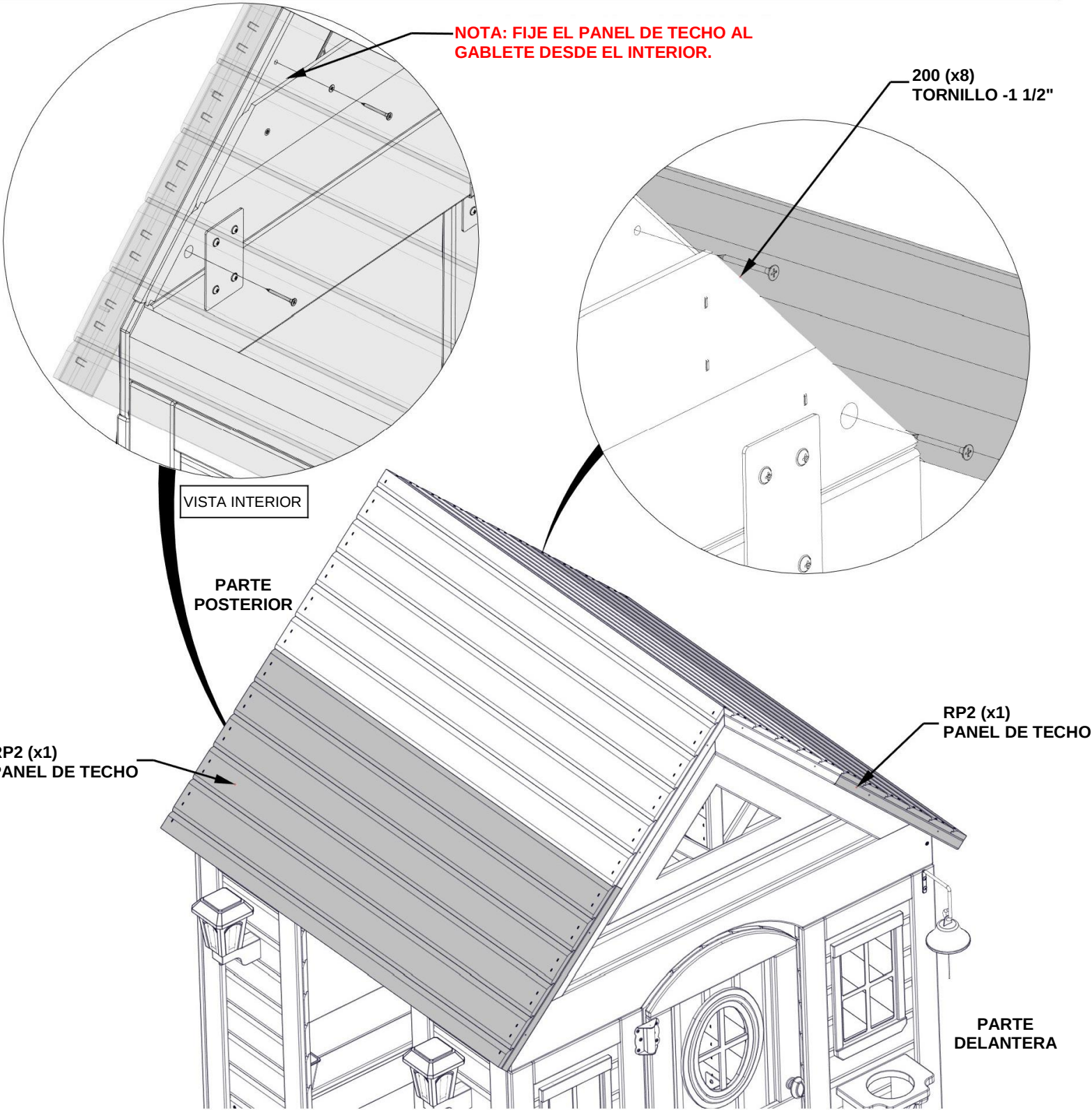
RP2 PANEL DE TECHO - W2A03587 (x2) 1 3/8"x17 7/8"x44 3/4" (35x454x1136)
