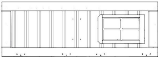
WP1 PANEL DE LA PARED - W2A03573 (x1) 3 3/8"x14"x39 3/4" (27x355x1010)
