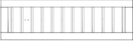
WP4 PANEL DE LA PARED - W2A03576 (x1) 1 1/16"x12 3/4"x41 5/8" (27x324x1058)
