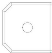
J6 SOPORTE DE VARILLA DE CORTINA (x1) INTERIOR - W4L17102 15/16"x2 3/8"x 2 3/8" (24x60x60)
