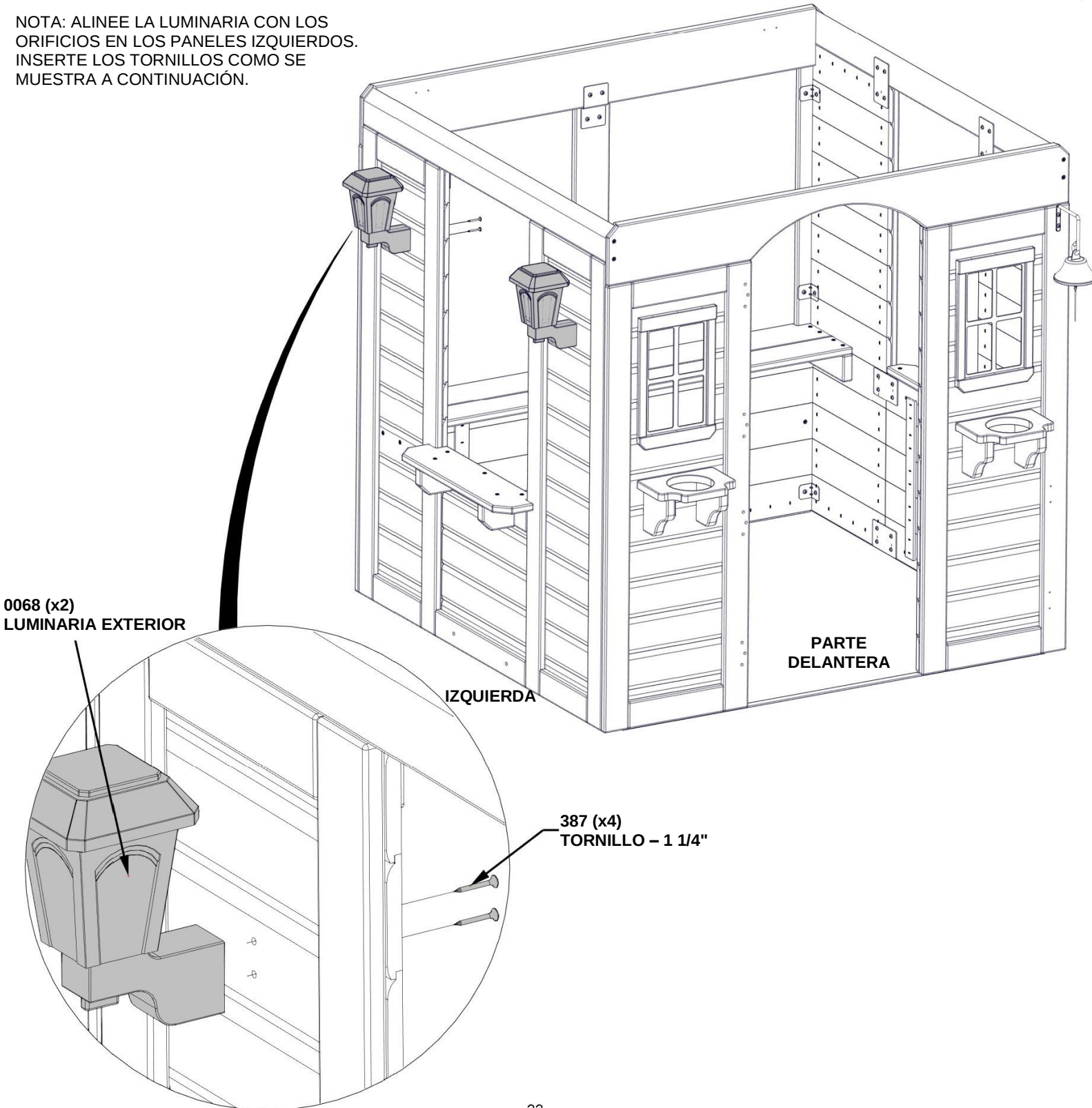
A6P00068 (x2) LUMINARIA EXTERIOR
