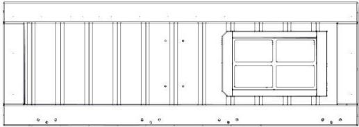
WP1 PANEL DE LA PARED - W2A03573 (x1) 3 3/8"x14"x39 3/4" (27x355x1010)
