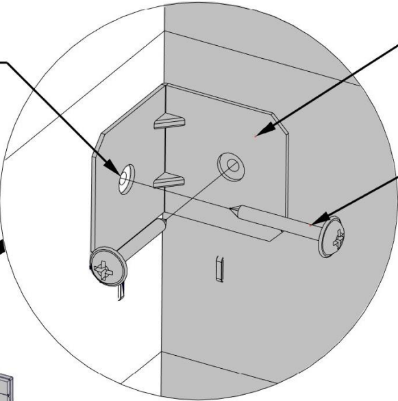
WP2 (x1) PANEL DE PARED
