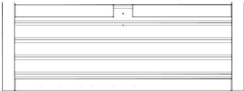
WP7 PANEL DE LA PARED - W2A03579 (x1) 1 1/4"x16 1/8"x42 7/8" (32x410x1088)
