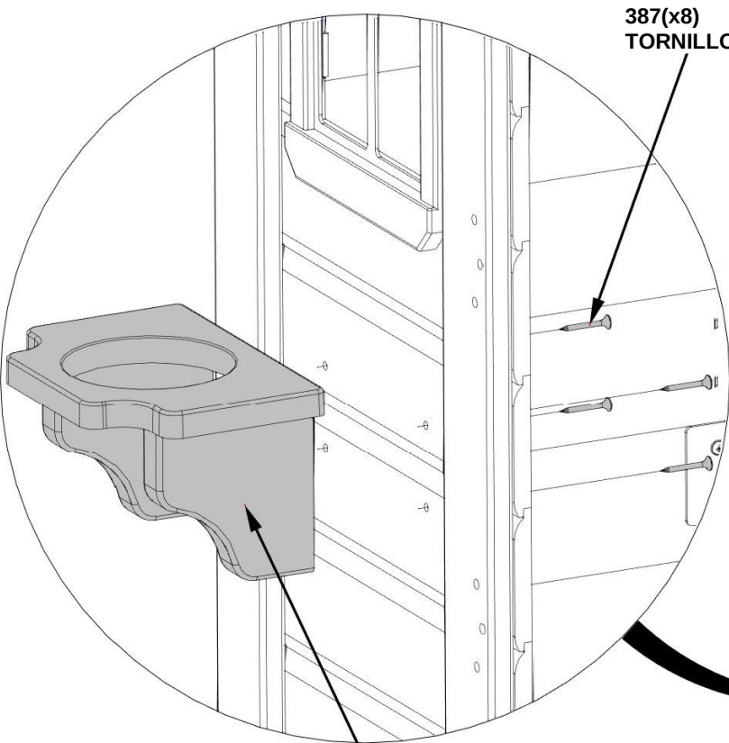
0023 (x2) PORTA MACETAS
