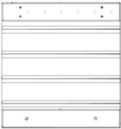
WP6 PANEL DE LA PARED - W2A03578 (x1) 1 1/4"x15 3/16"x16 1/8" (32x386x410)
