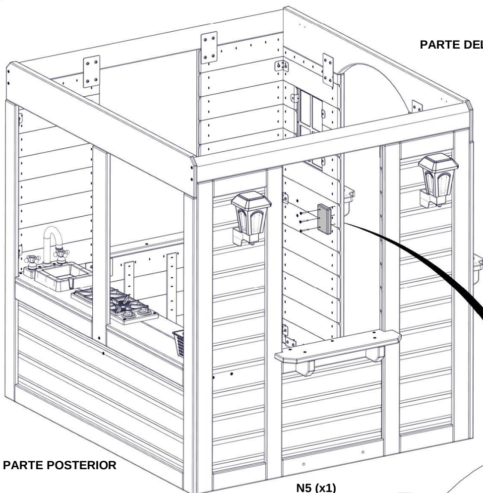
N5 TOPE DE PUERTA - W4L17348 (x1) 5/8"x2 3/8"x3 3/8" (16x60x86)
