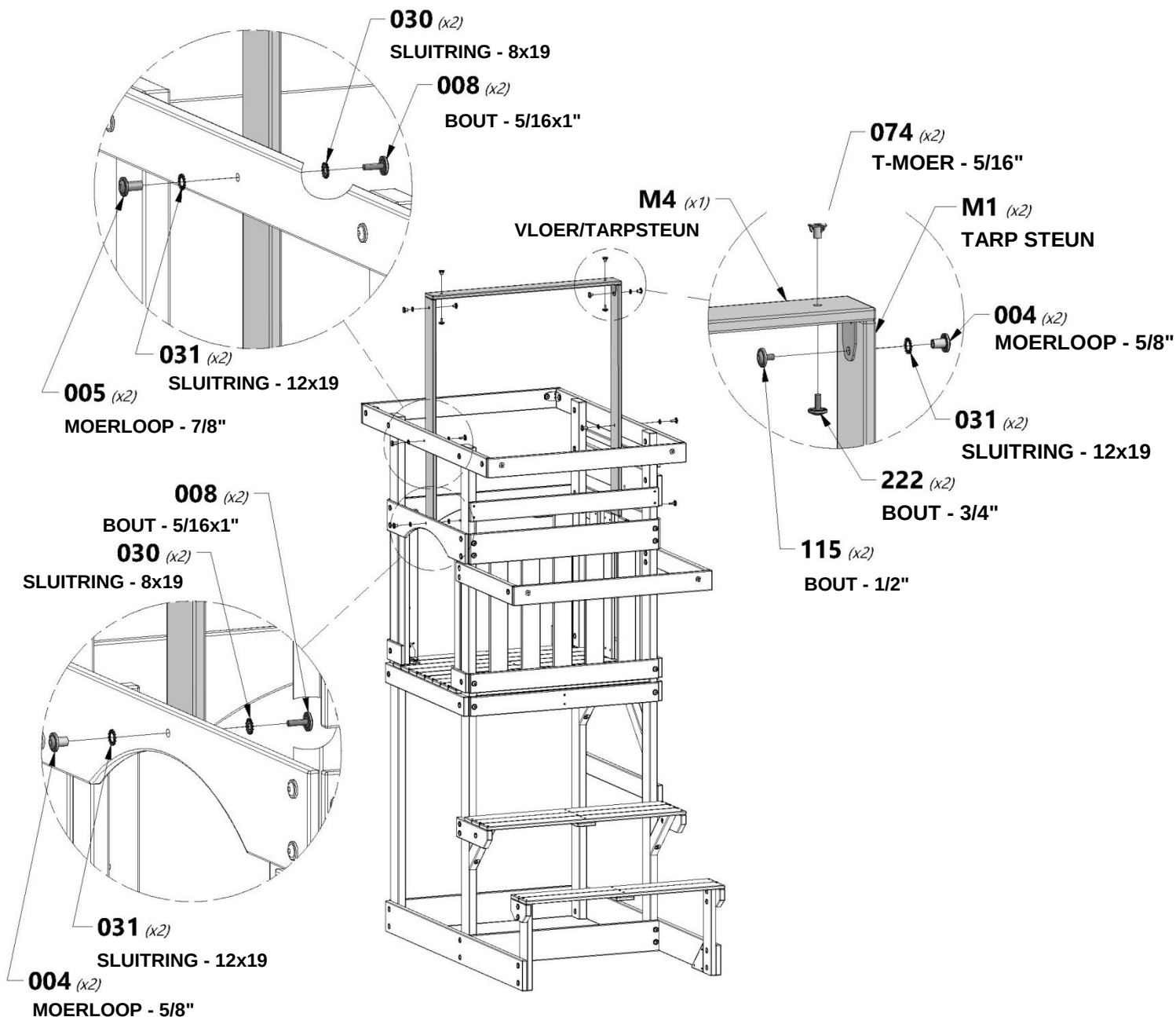
H100031 | SLUITRING VERGRENDING EXTERN 12x19 (6)
