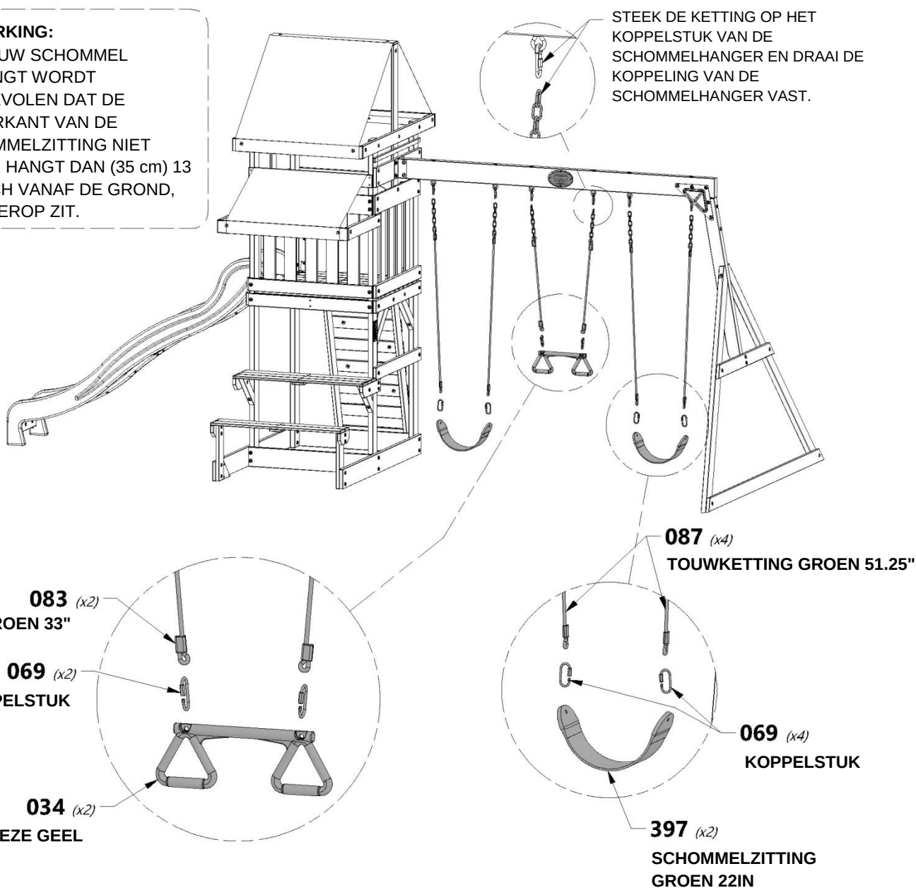
A100087 (4) | TOUWKETTING GROEN 51.25"
