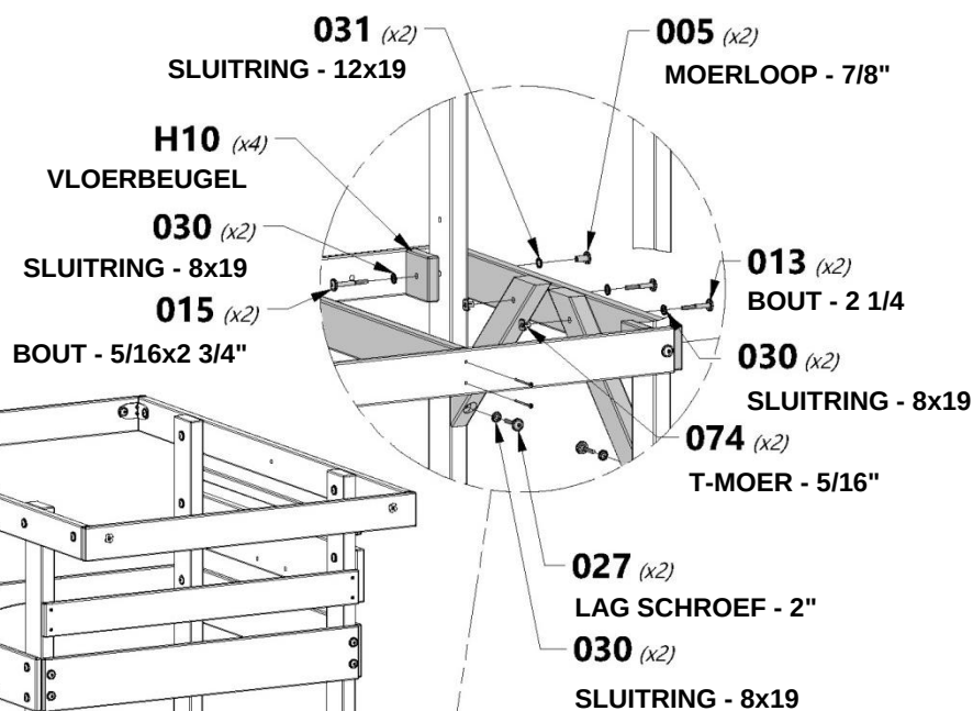
H100030 | SLUITRING VERGREDELING EXTERN (8) | 8x19
