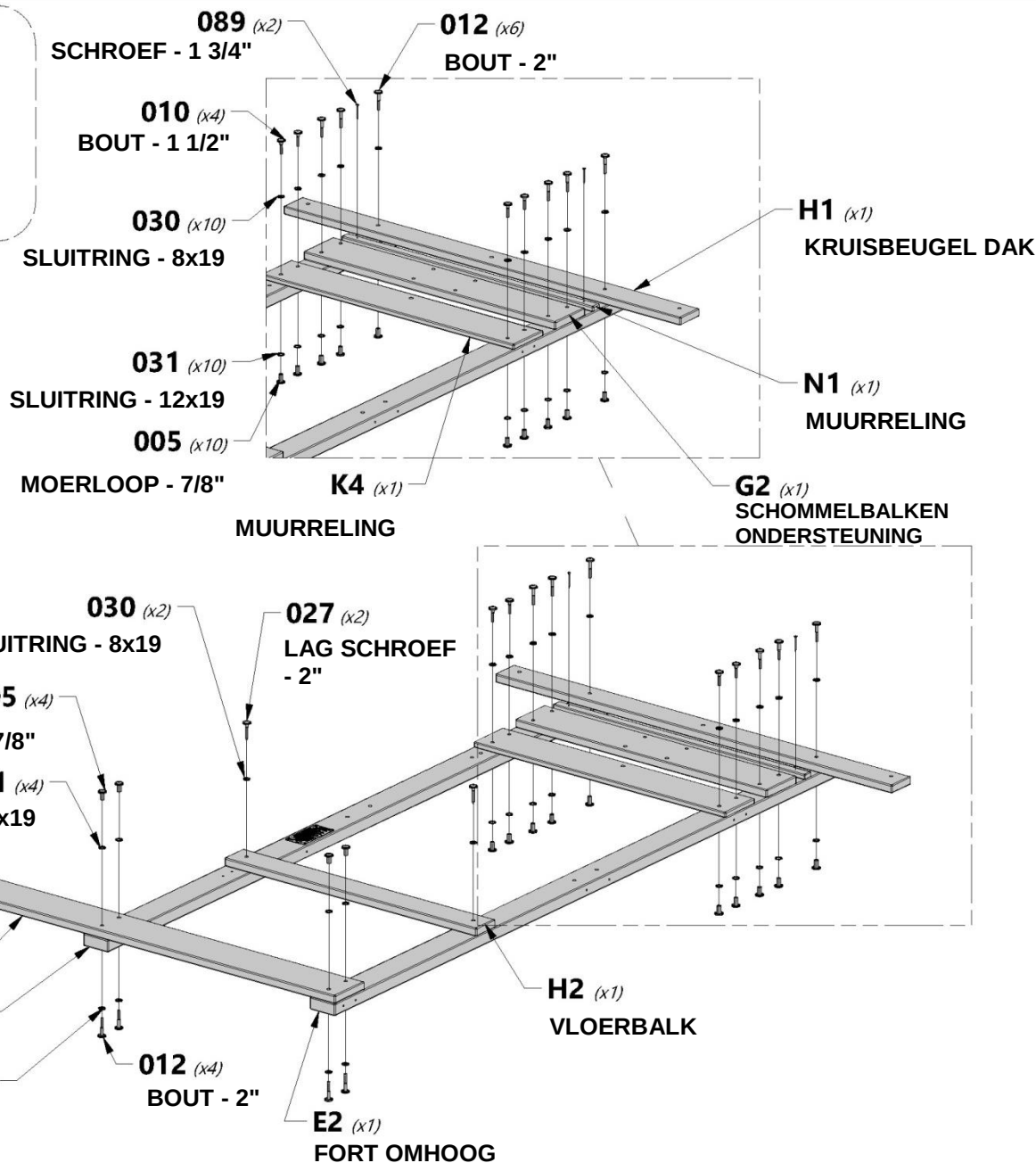
H100089 SCHROEF PFH (2) 8x1 3/4
